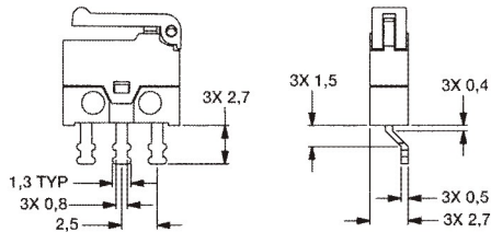
SMT Mounting Pattern
